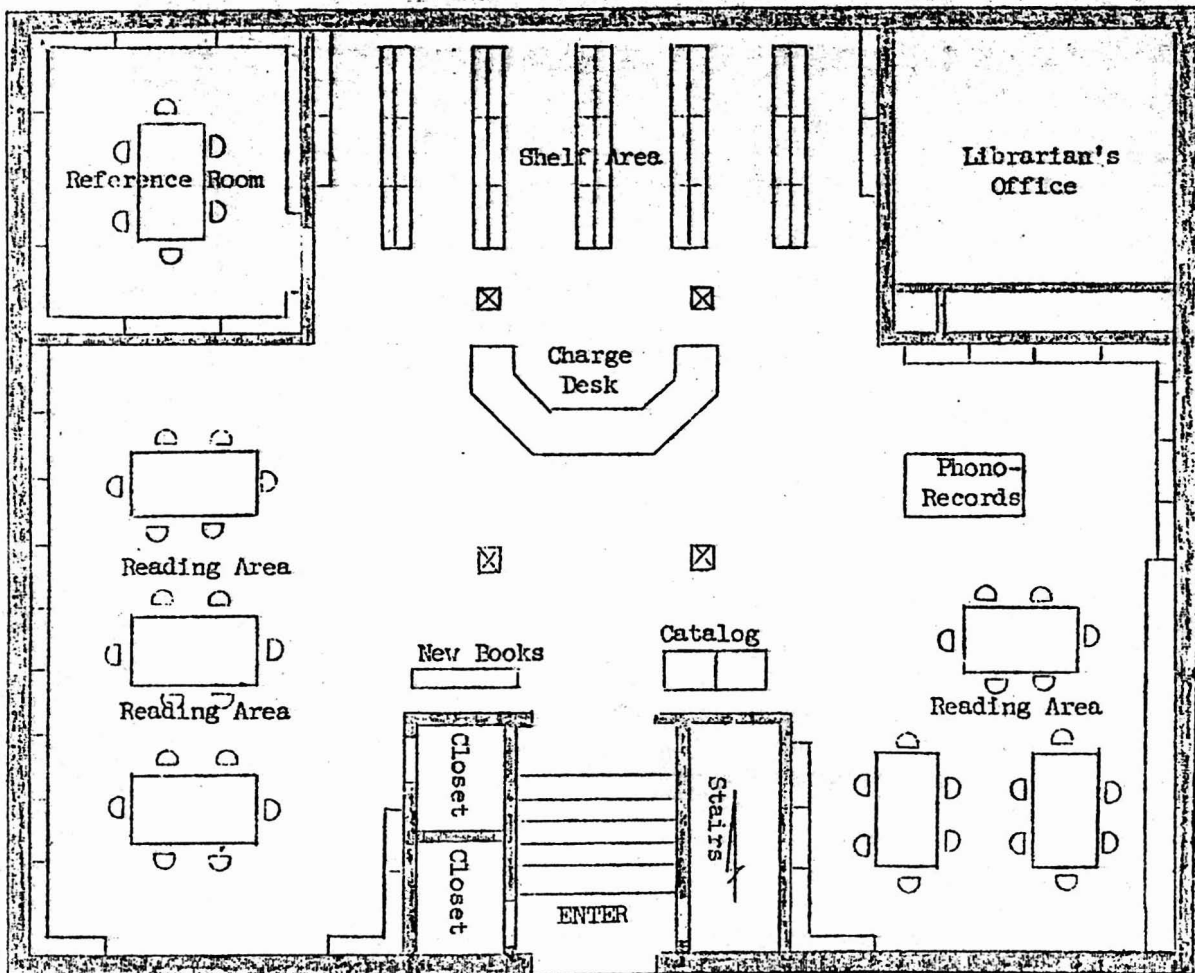
Figure 3. Arrangement of Floor Area, Livermore Public Library, 1961.
